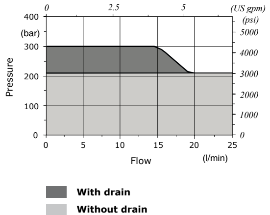
Minimum dynamic conditions (Supply = Vn-10%, coil at 70 °C - 158 °F)
