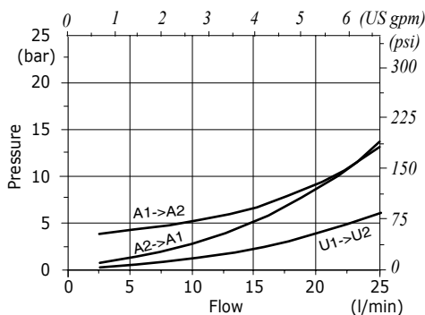
VBPSL/R..14 pressure drop vs. flow
